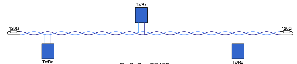
Fig 9: Bus RS485
